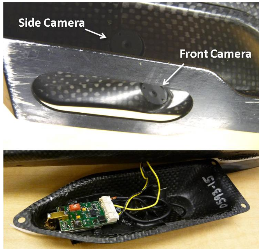
Figure 9. BATCAM CCD Cameras and Camera Pod
