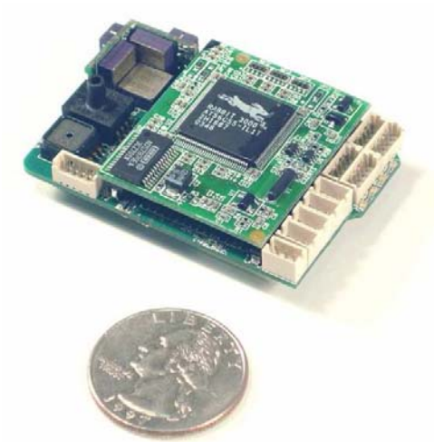
Figure 8. Procerus Technologies Kestrel™ Autopilot [47]
