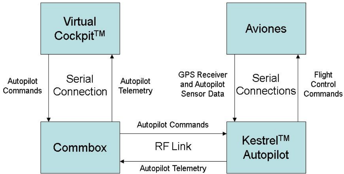
Figure 15. Hardware-in-the-Loop Setup
