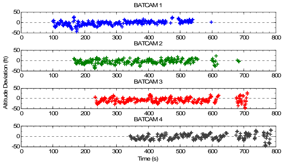
Figure 38. Altitude Deviations
