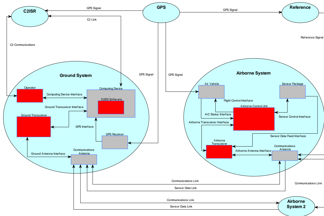
Figure 30. CUSS SV-1 System Interface Description
